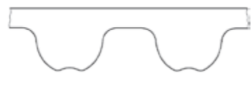
optibelt OMEGA HP in cross section
