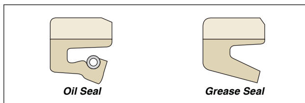
Figure 2-4. Oil and Grease Seals
