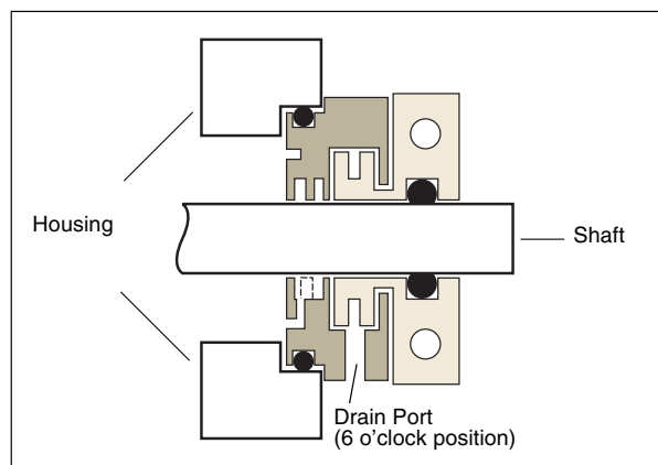
Figure 8-3. Proper Installation
