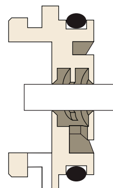
ProTech Stator
