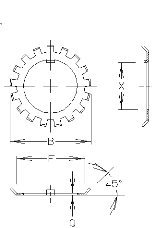
Figure 2 – Lockwashers
